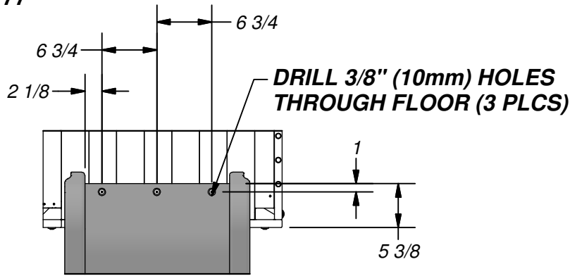
SLIDE ASSEMBLY
